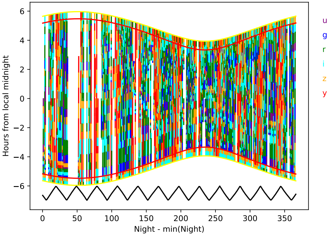
ddf_acor_sf25_lsf30_lsr50_v3.4_10yrs year 2-3: Hourglass
