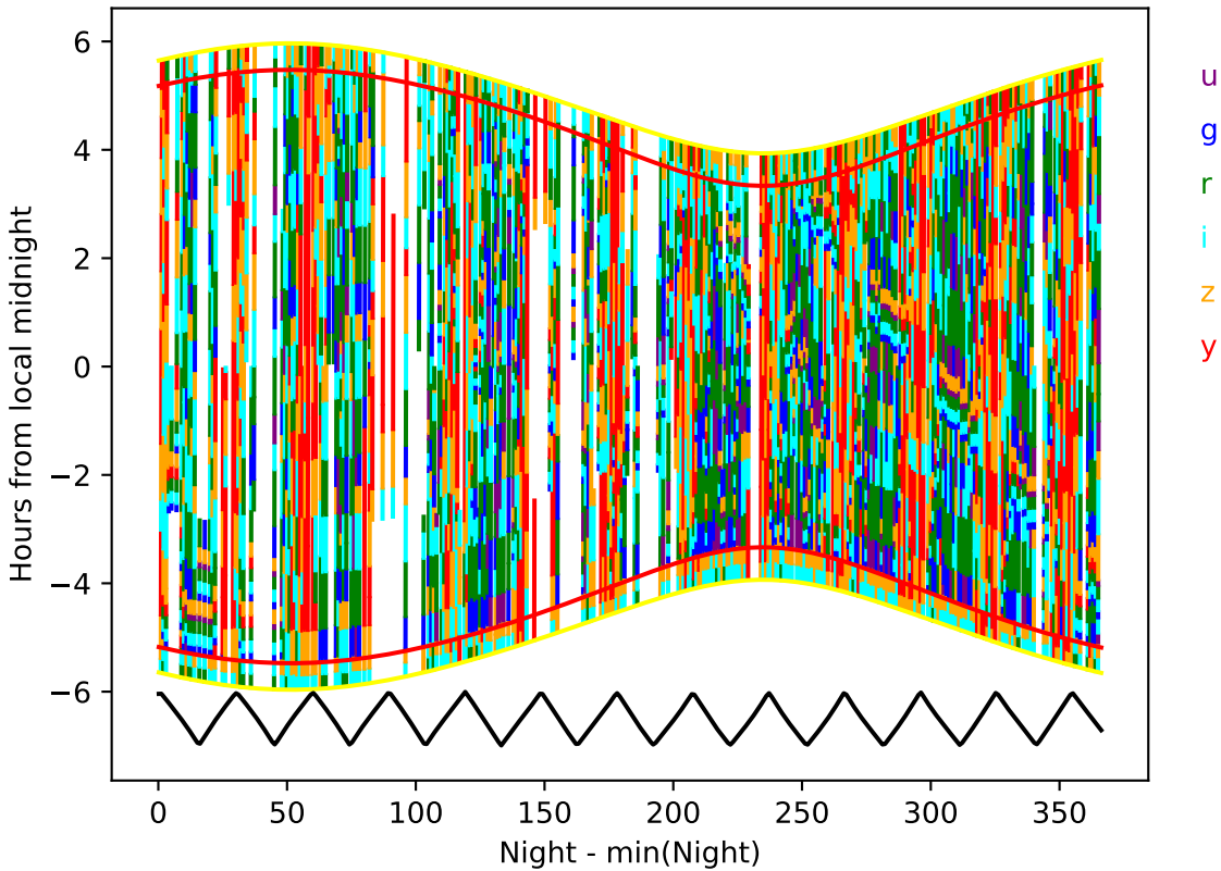
ddf_acor_sf25_lsf30_lsr50_v3.4_10yrs year 1-2: Hourglass
