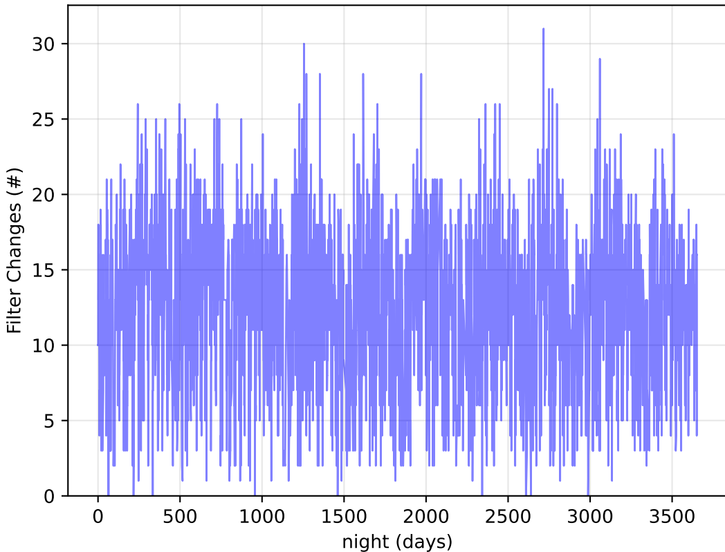
ddf_acor_sf25_lsf30_lsr50_v3.4_10yrs : Filter Changes
