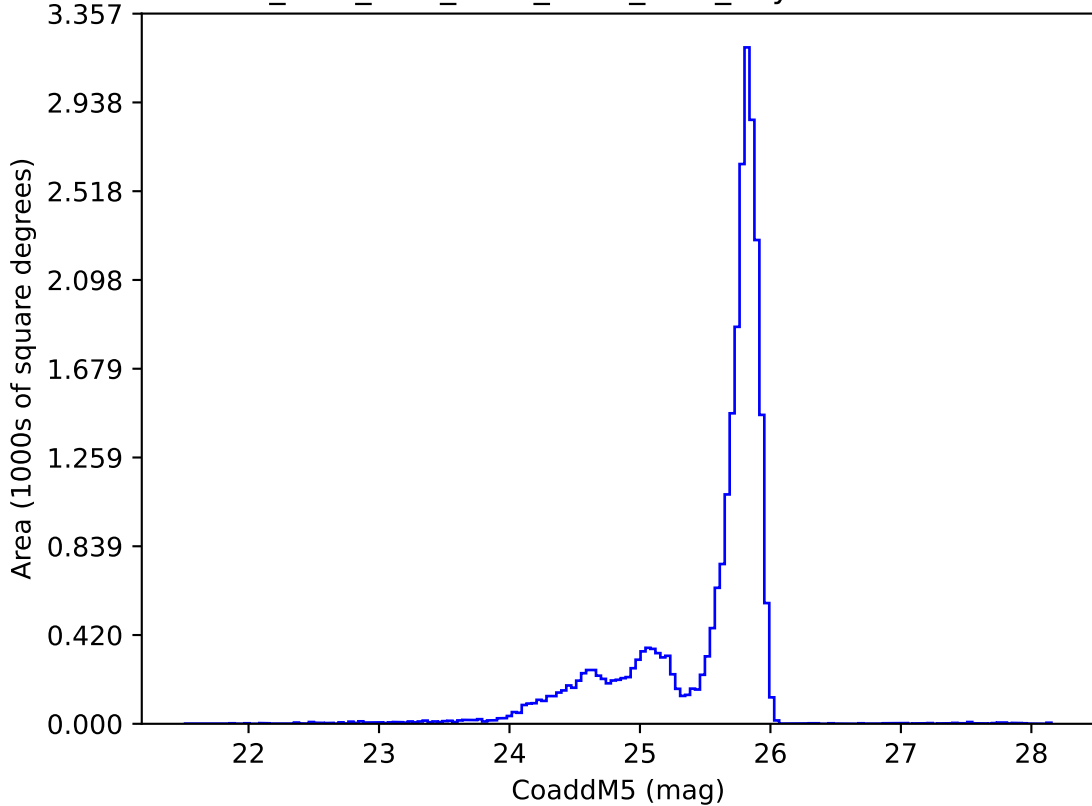
ddf_acor_sf25_lsf30_lsr50_v3.4_10yrs z: CoaddM5
