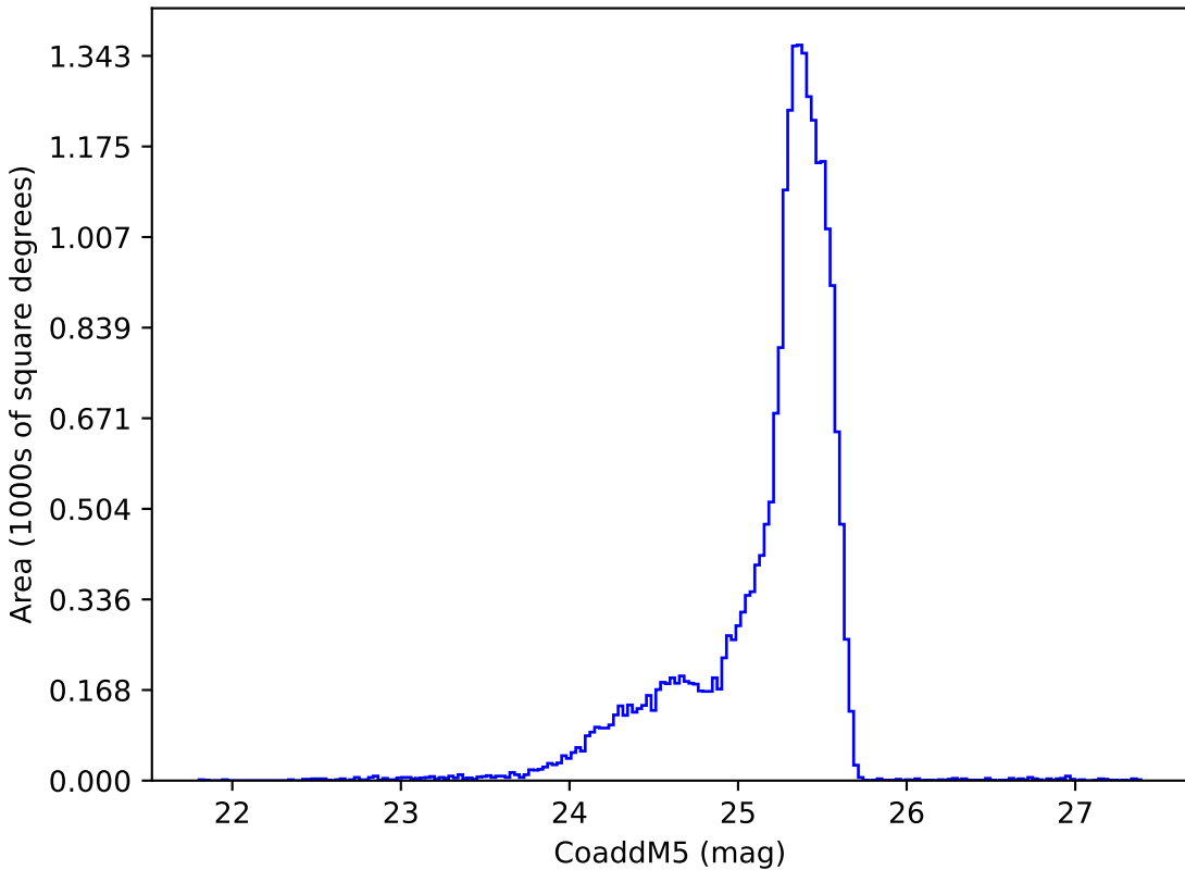
ddf_acor_sf25_lsf30_lsr50_v3.4_10yrs u: CoaddM5
