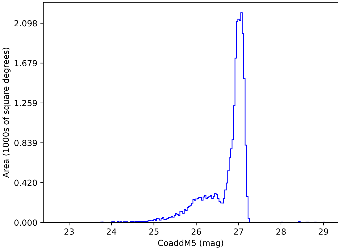
ddf_acor_sf25_lsf30_lsr50_v3.4_10yrs r: CoaddM5
