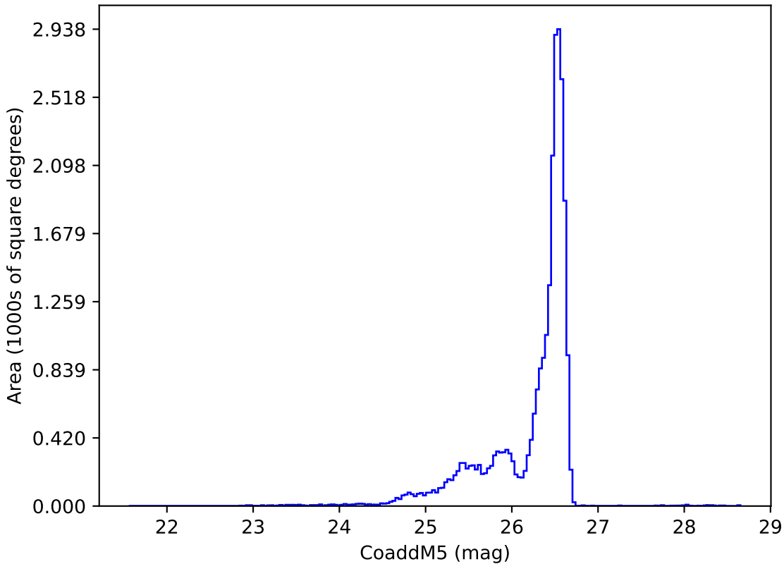
ddf_acor_sf25_lsf30_lsr50_v3.4_10yrs i: CoaddM5
