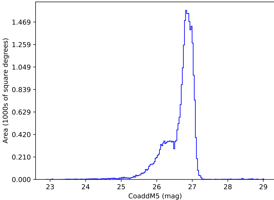
ddf_acor_sf25_lsf30_lsr50_v3.4_10yrs g: CoaddM5
