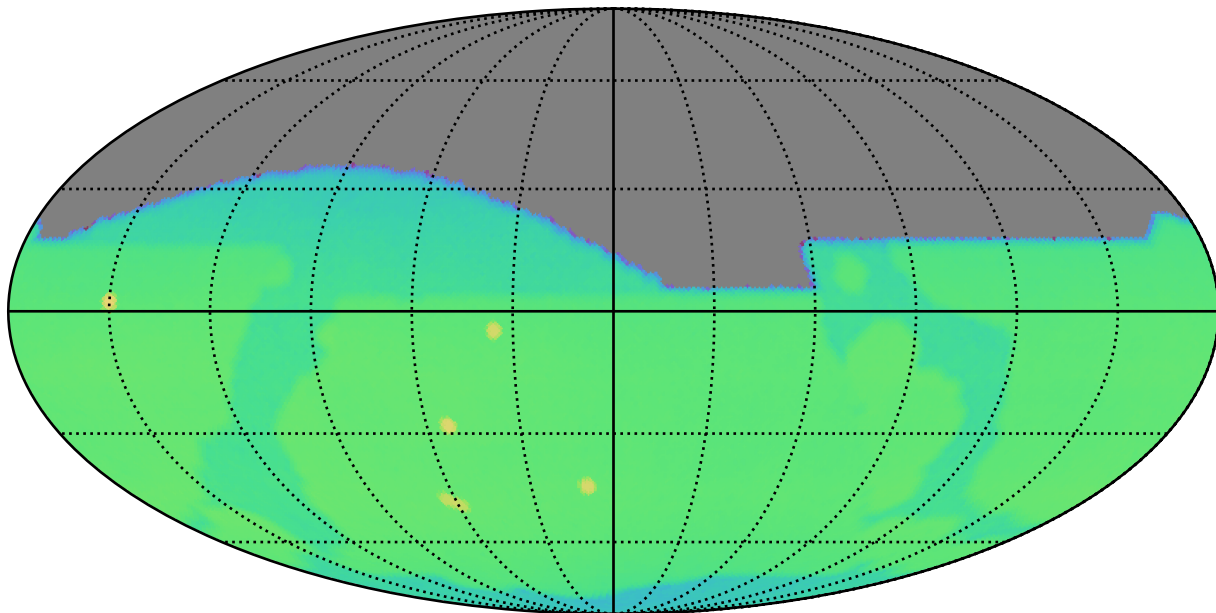
ddf_acor_sf25_lsf30_lsr50_v3.4_10yrs : CoaddM5
