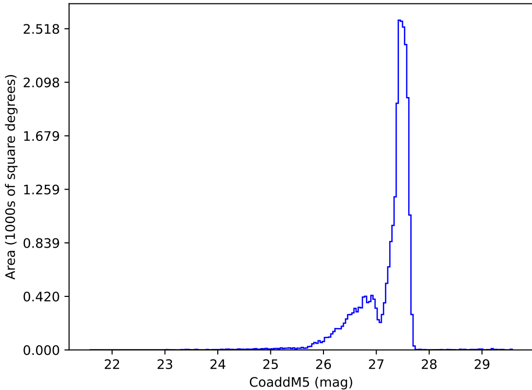
ddf_acor_sf25_lsf30_lsr50_v3.4_10yrs : CoaddM5
