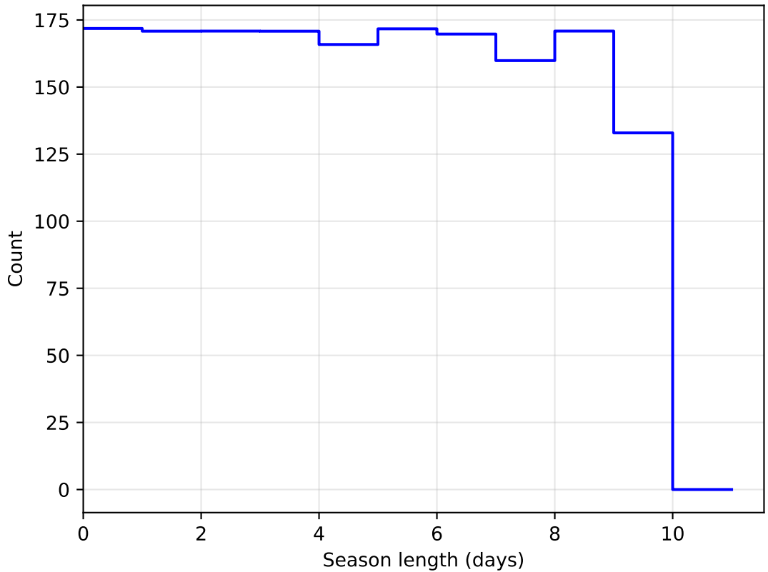
ddf_acor_sf25_lsf30_lsr50_v3.4_10yrs DD:ECDFS all bands: SeasonLength
