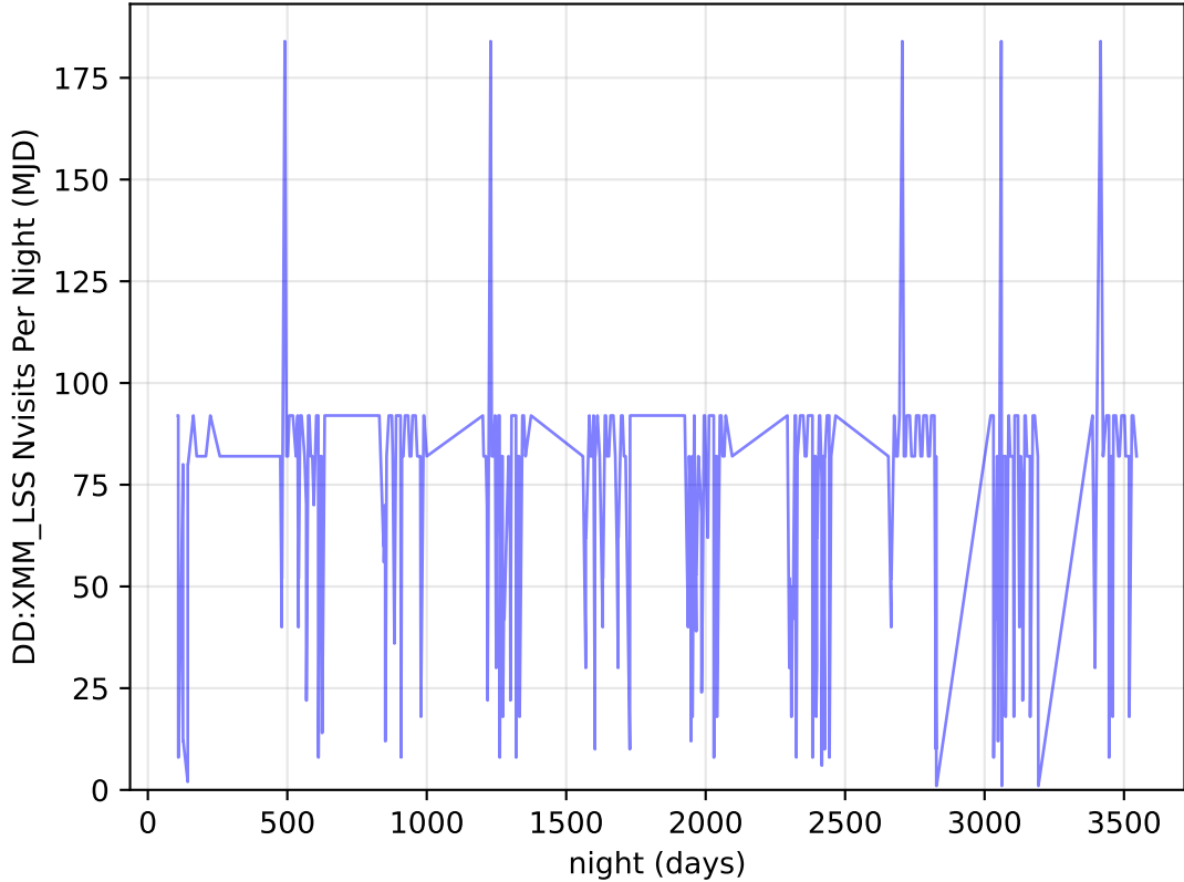
ddf_acor_sf25_lsf30_lsr50_v3.4_10yrs all bands: DD:XMM_LSS Nvisits Per Night
