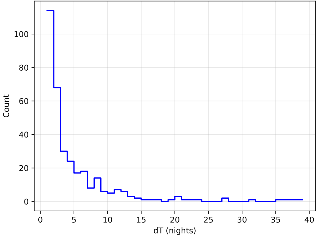
ddf_acor_sf25_lsf30_lsr50_v3.4_10yrs all bands: DD:WFD Delta Nights Histogram
