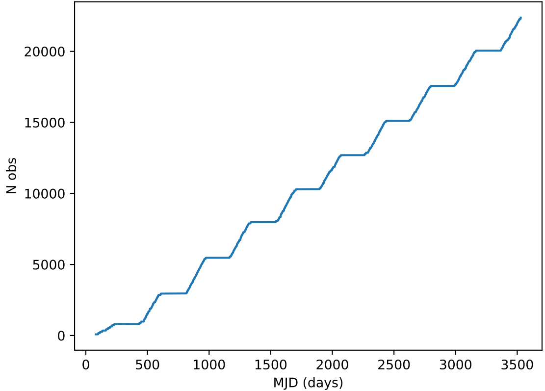
ddf_acor_sf25_lsf30_lsr50_v3.4_10yrs all bands: DD:ELAISS1 Cumulative NVisits
