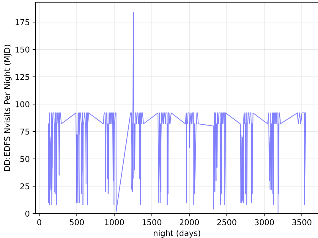
ddf_acor_sf25_lsf30_lsr50_v3.4_10yrs all bands: DD:EDFS Nvisits Per Night
