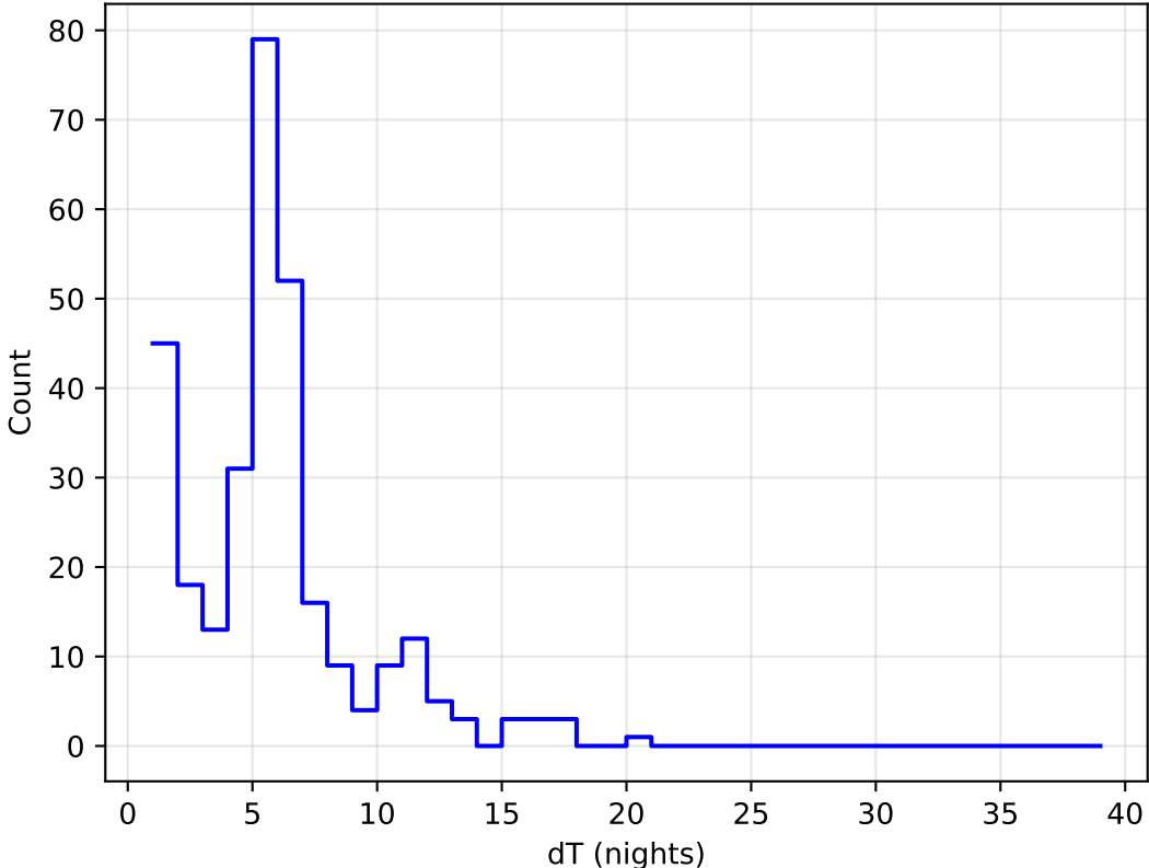
ddf_acor_sf25_lsf30_lsr50_v3.4_10yrs all bands: DD:EDFS Delta Nights Histogram
