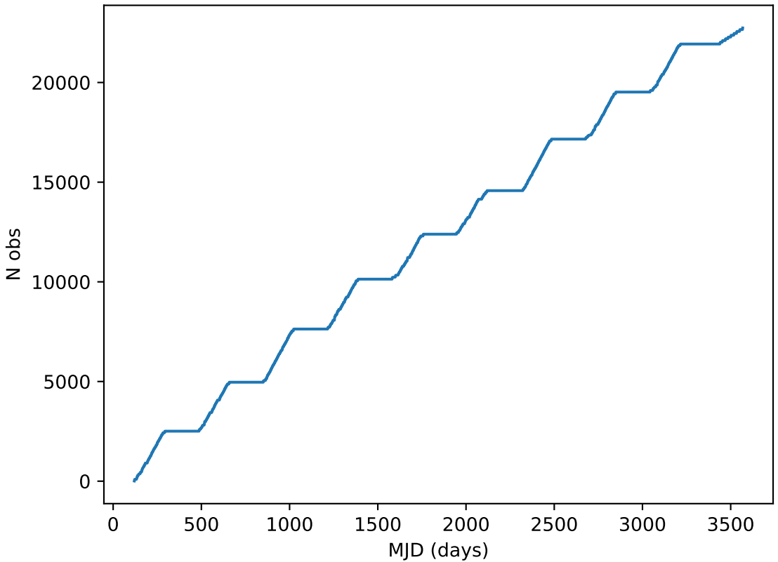
ddf_acor_sf25_lsf30_lsr50_v3.4_10yrs all bands: DD:EDFS Cumulative NVisits
