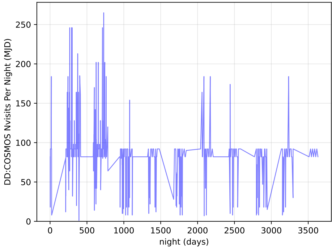
ddf_acor_sf25_lsf30_lsr50_v3.4_10yrs all bands: DD: COSMOS Nvisits Per Night
