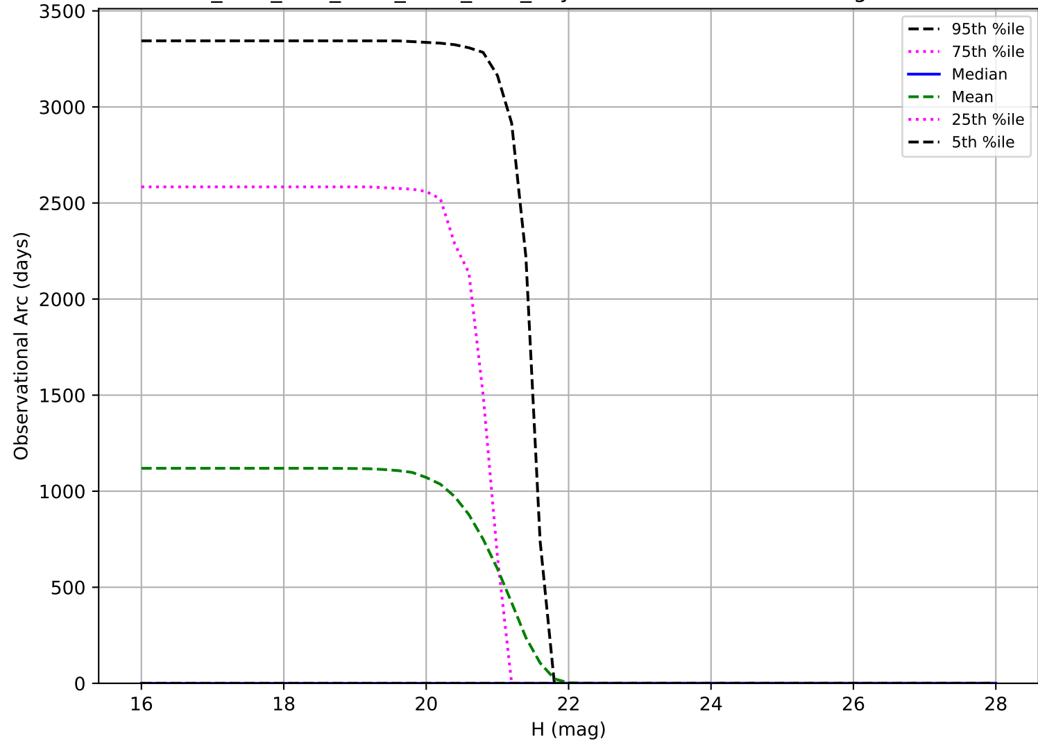
ddf_acor_sf25_lsf30_lsr20_v3.4_10yrs: Observational Arc Length Vatira
