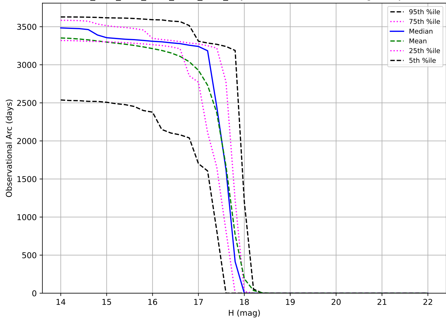
ddf_acor_sf25_lsf30_lsr20_v3.4_10yrs: Observational Arc Length Trojan
