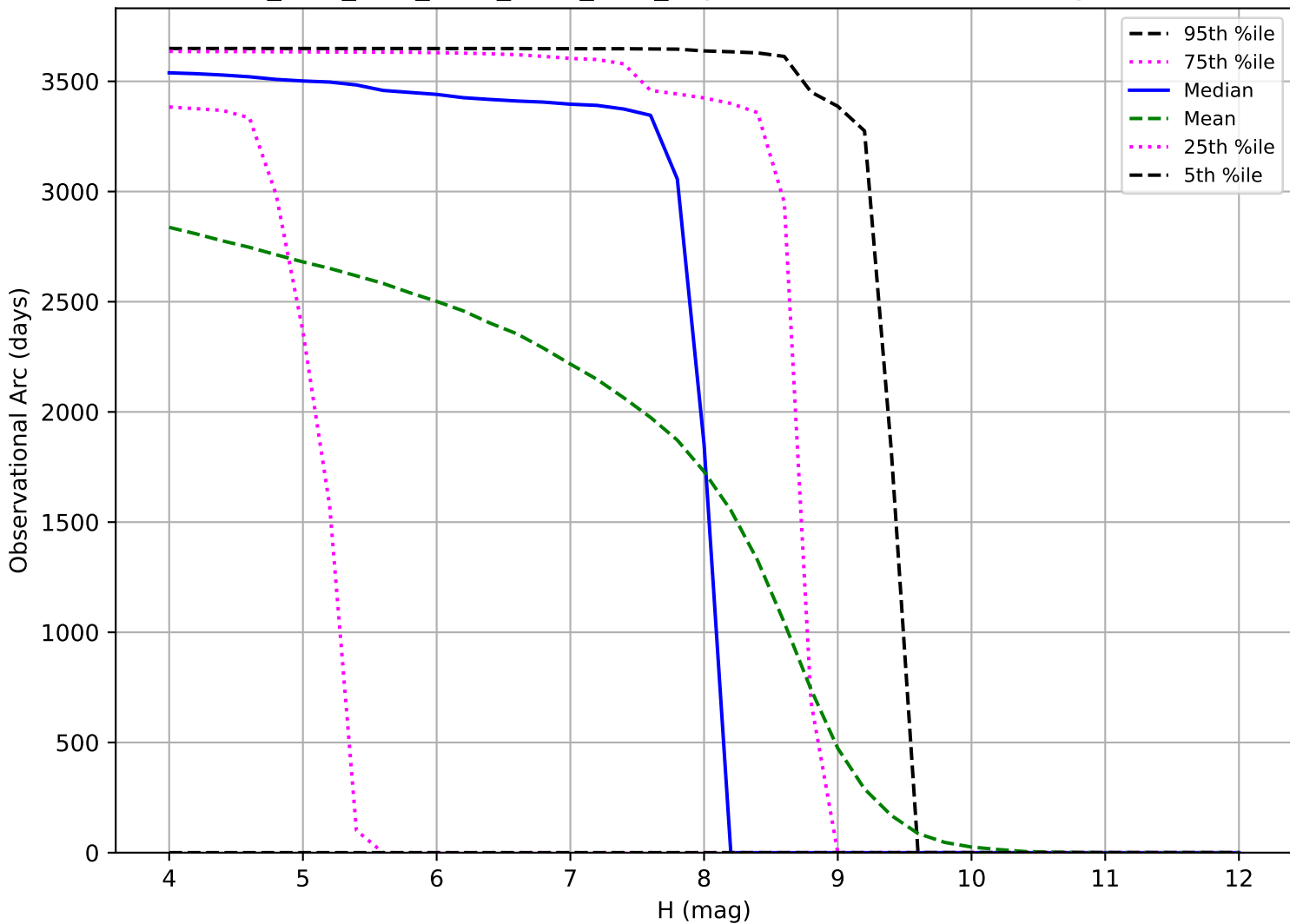
ddf_acor_sf25_Isf30_Isr20_v3.4_10yrs: Observational Arc Length TNO
