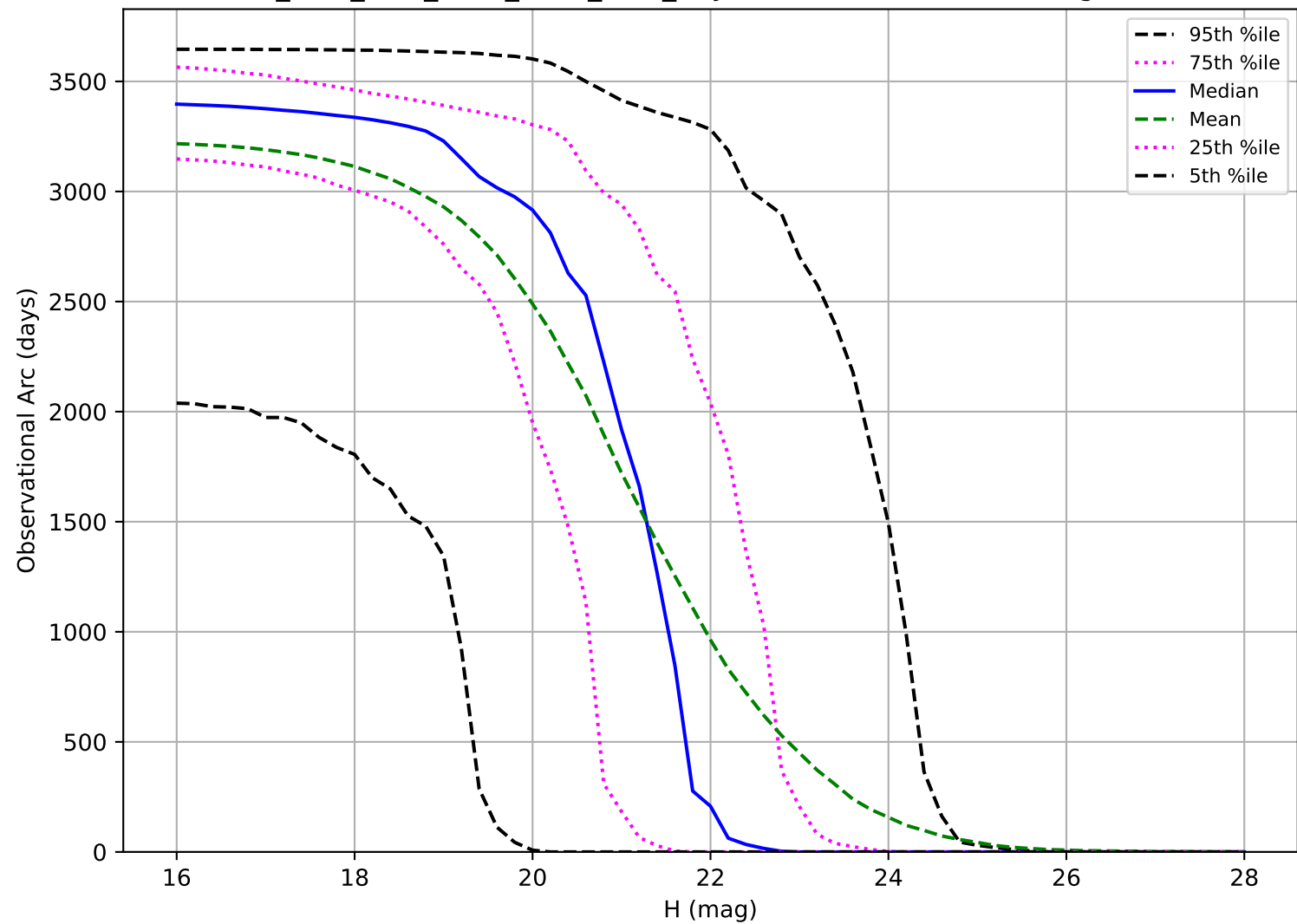
ddf_acor_sf25_lsf30_lsr20_v3.4_10yrs: Observational Arc Length PHA
