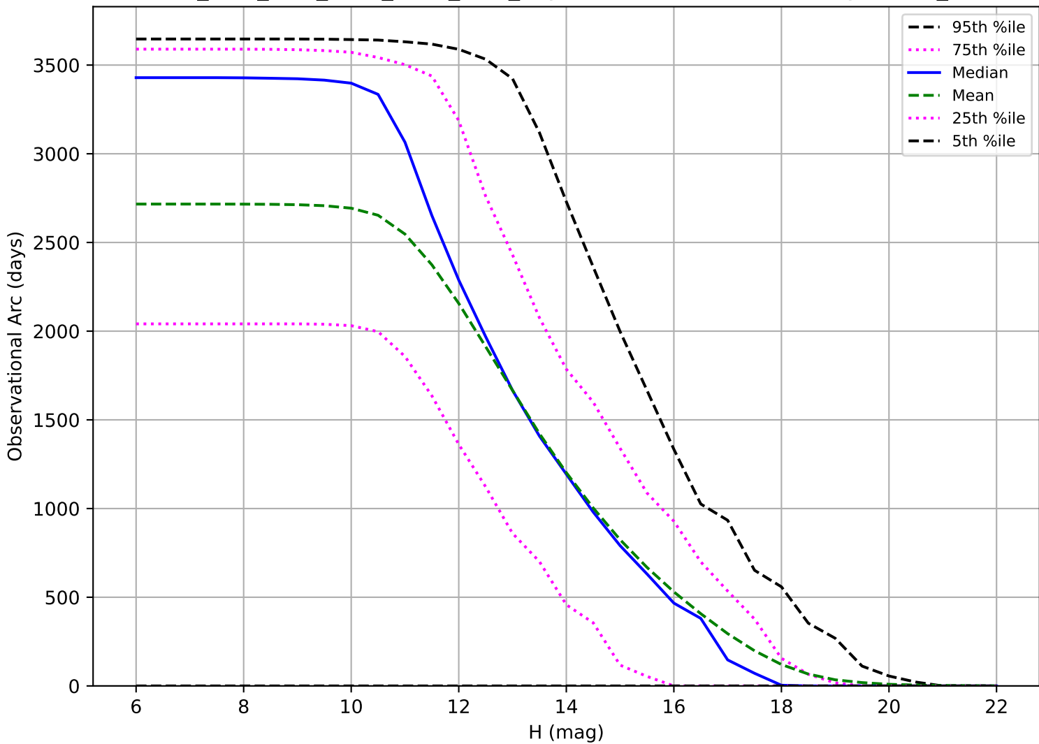
ddf_acor_sf25_lsf30_lsr20_v3.4_10yrs: Observational Arc Length OCC_r5
