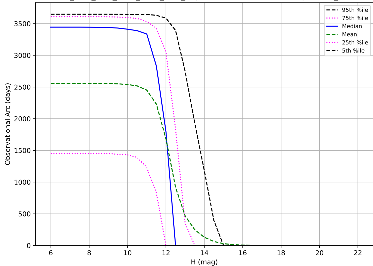
ddf_acor_sf25_lsf30_lsr20_v3.4_10yrs: Observational Arc Length OCC_r20
