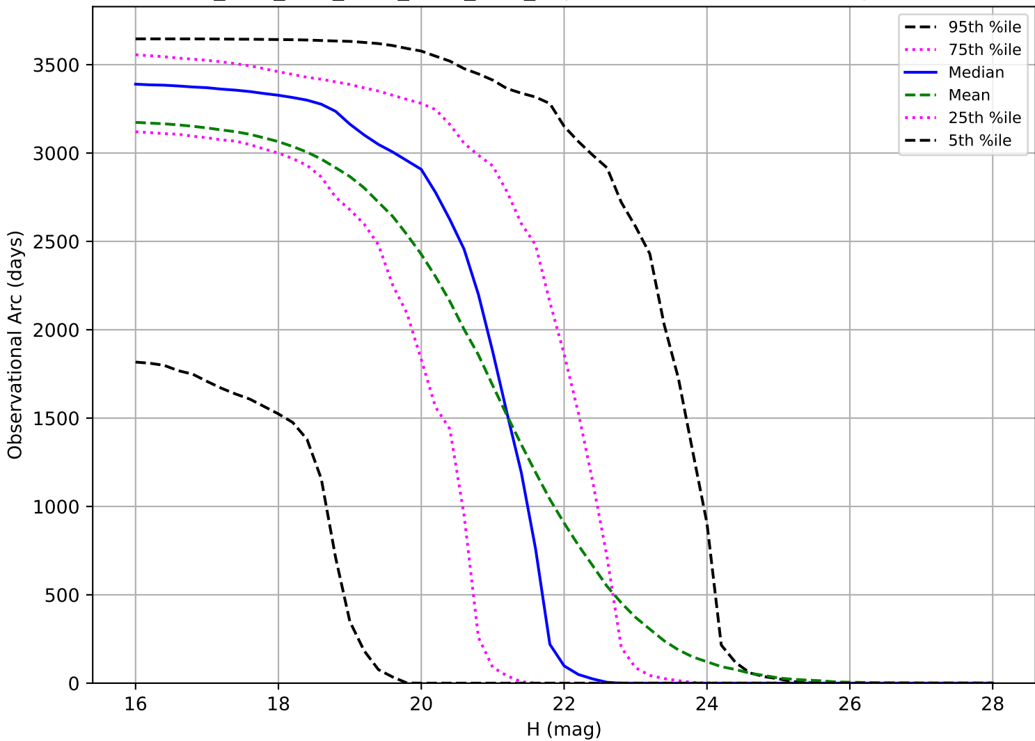
ddf_acor_sf25_lsf30_lsr20_v3.4_10yrs: Observational Arc Length NEO
