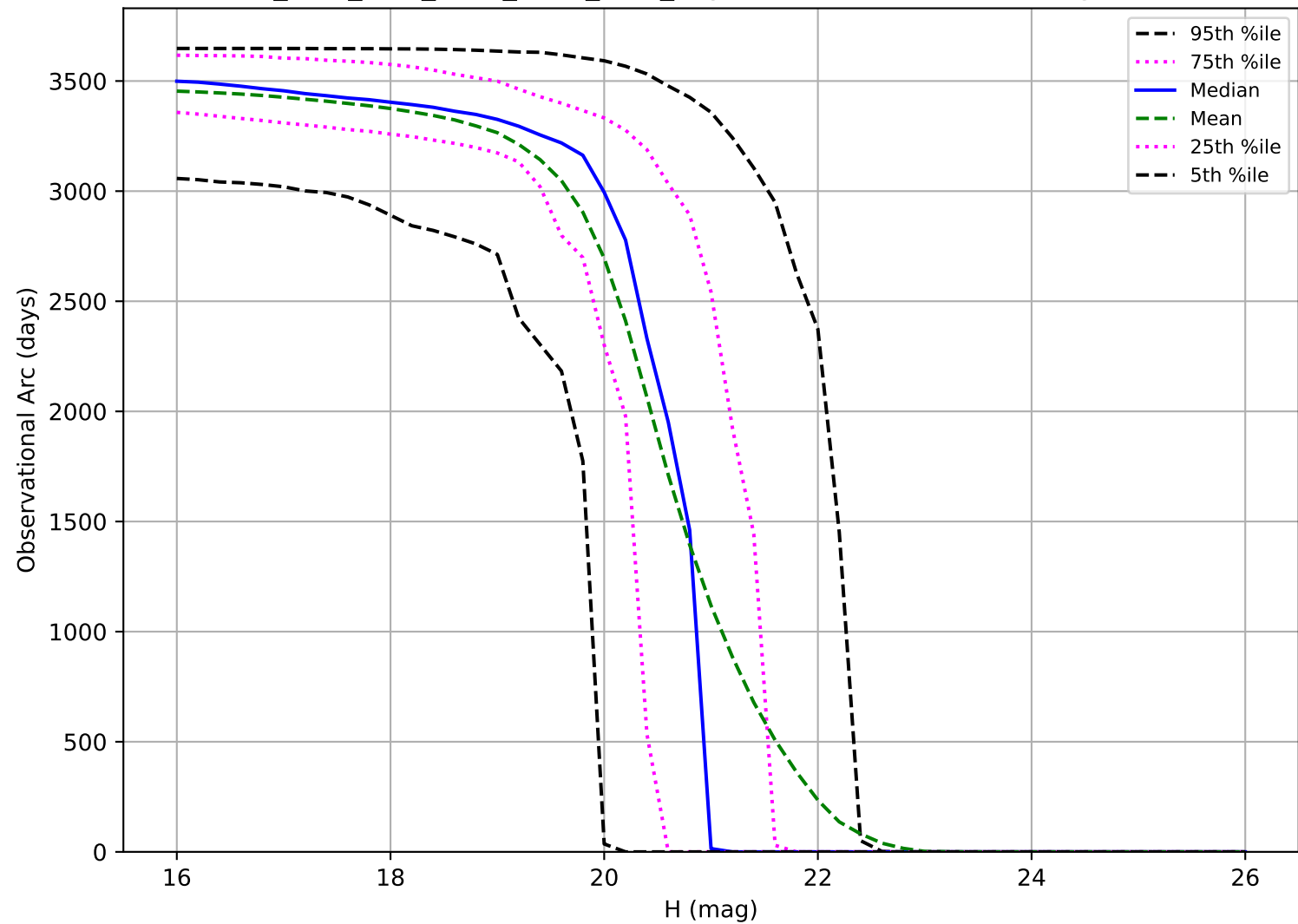
ddf_acor_sf25_lsf30_lsr20_v3.4_10yrs: Observational Arc Length MBA
