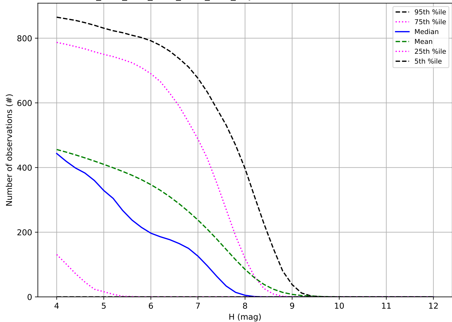
ddf_acor_sf25_lsf30_lsr20_v3.4_10yrs: Number of observations TNO
