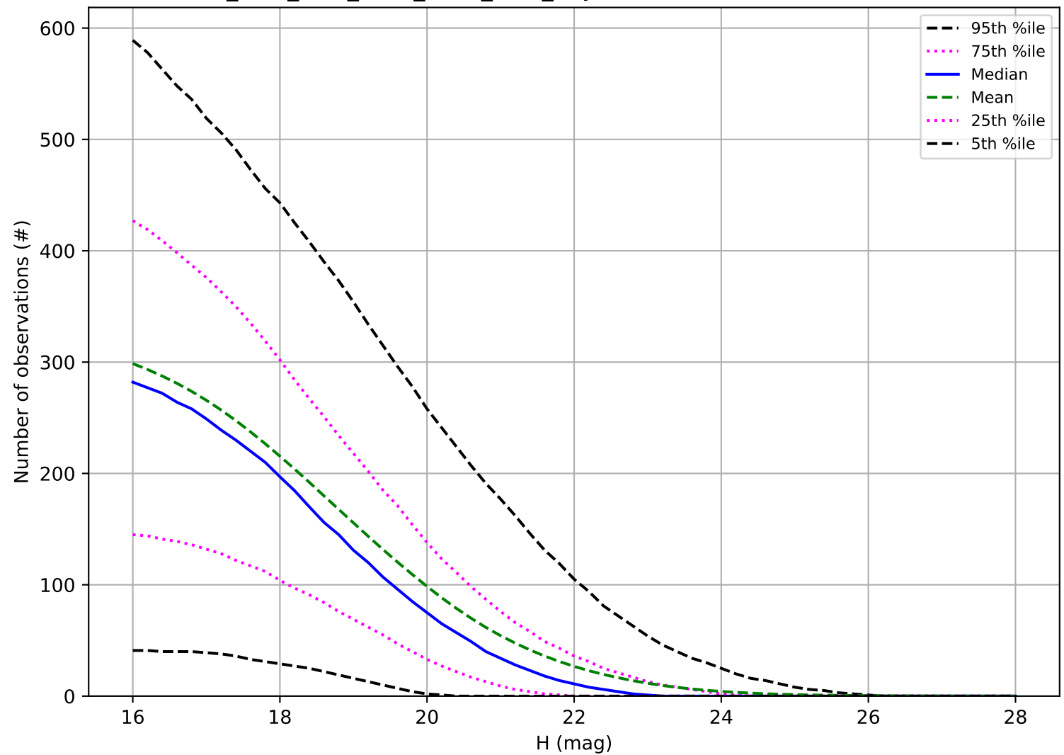
ddf_acor_sf25_lsf30_lsr20_v3.4_10yrs: Number of observations PHA
