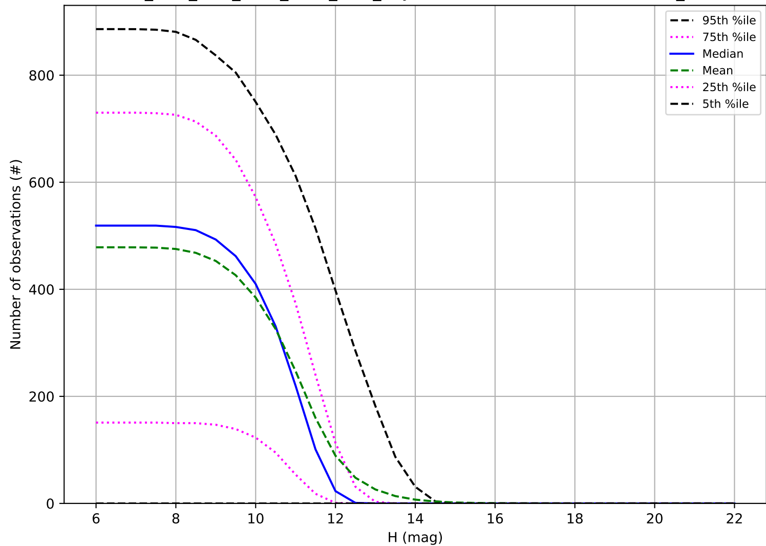
ddf_acor_sf25_lsf30_lsr20_v3.4_10yrs: Number of observations OCC_r20
