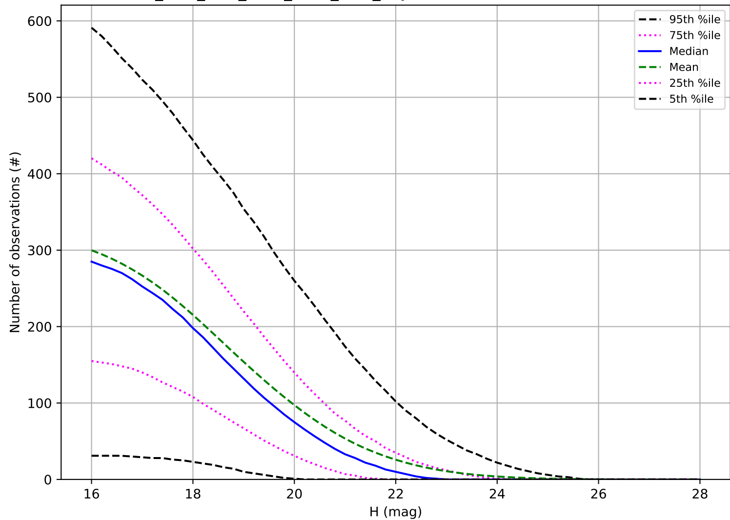
ddf_acor_sf25_lsf30_lsr20_v3.4_10yrs: Number of observations NEO
