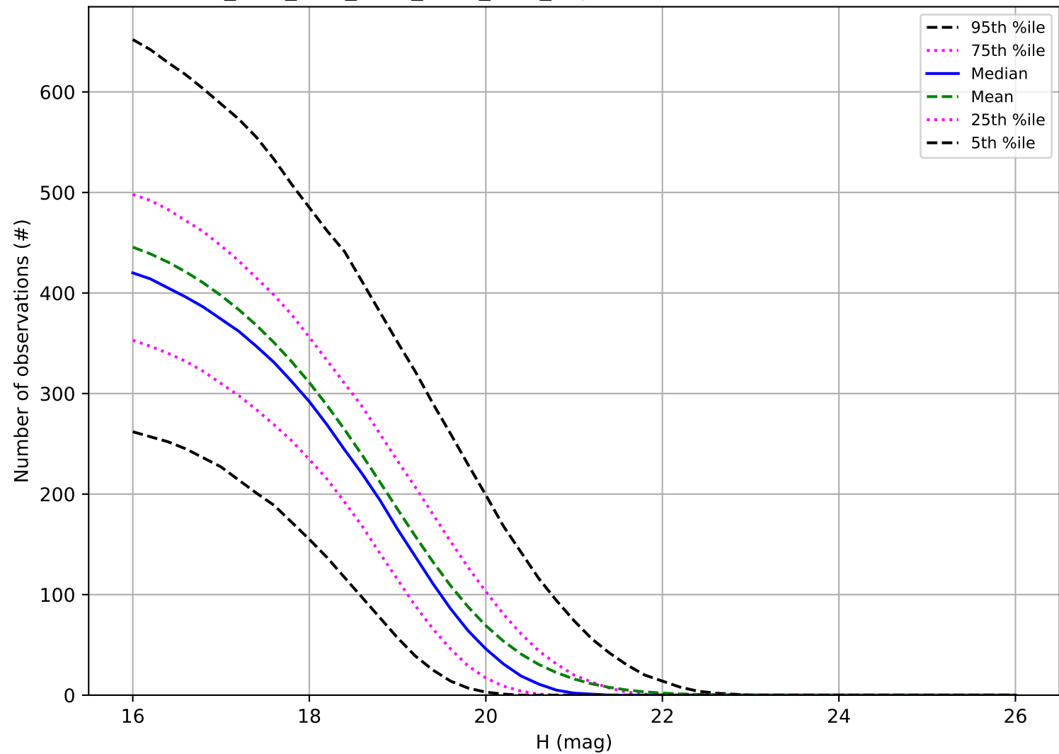
ddf_acor_sf25_lsf30_lsr20_v3.4_10yrs: Number of observations MBA
