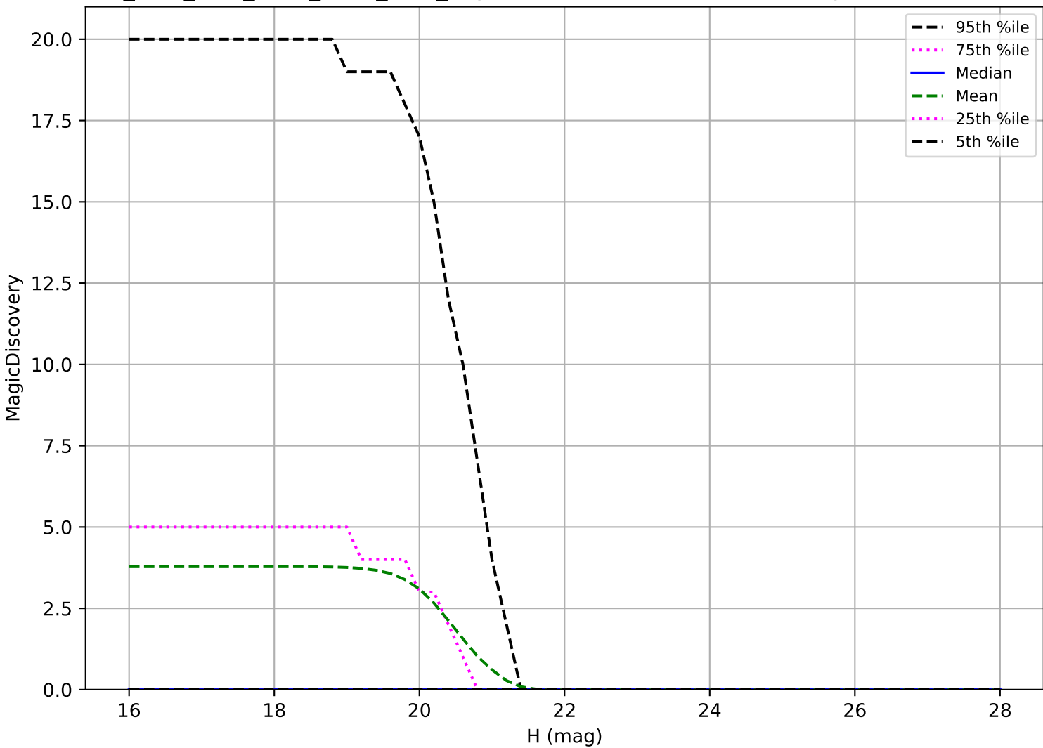
ddf_acor_sf25_lsf30_lsr20_v3.4_10yrs: Vatra 6 detections in 60 nights detection loss
