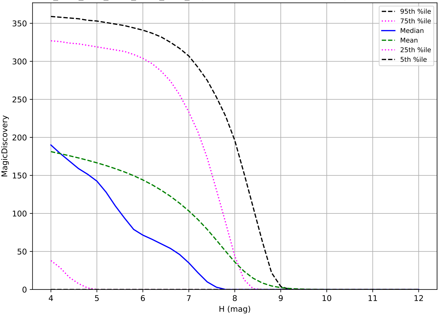
ddf_acor_sf25_lsf30_lsr20_v3.4_10yrs: TNO 6 detections in 60 nights detection loss
