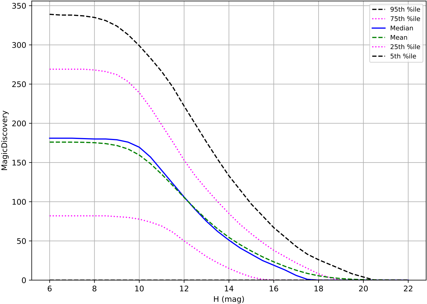
ddf_acor_sf25_lsf30_lsr20_v3.4_10yrs: OCC_r5 6 detections in 60 nights detection loss
