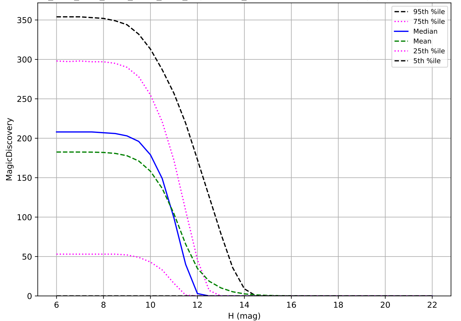
ddf_acor_sf25_lsf30_lsr20_v3.4_10yrs: OCC_r20 6 detections in 60 nights detection loss
