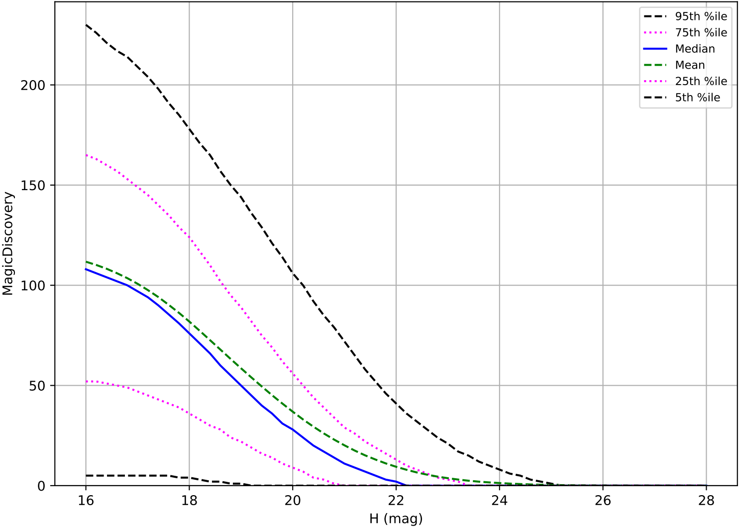
ddf_acor_sf25_lsf30_lsr20_v3.4_10yrs: NEO 6 detections in 60 nights detection loss
