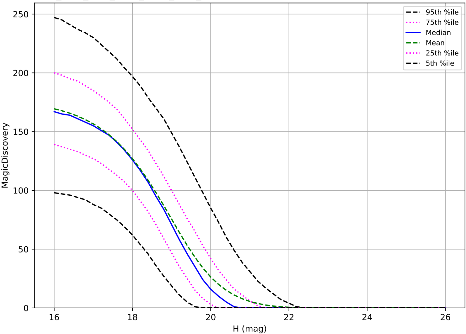
ddf_acor_sf25_lsf30_lsr20_v3.4_10yrs: MBA 6 detections in 60 nights detection loss
