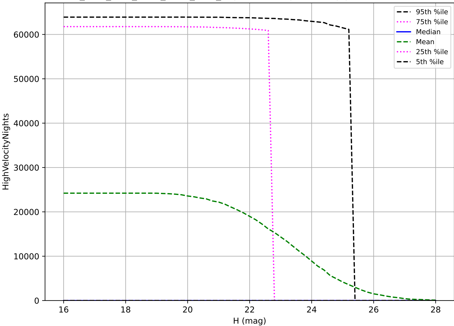
ddf_acor_sf25_lsf30_lsr20_v3.4_10yrs: PHA High velocity pair detection loss
