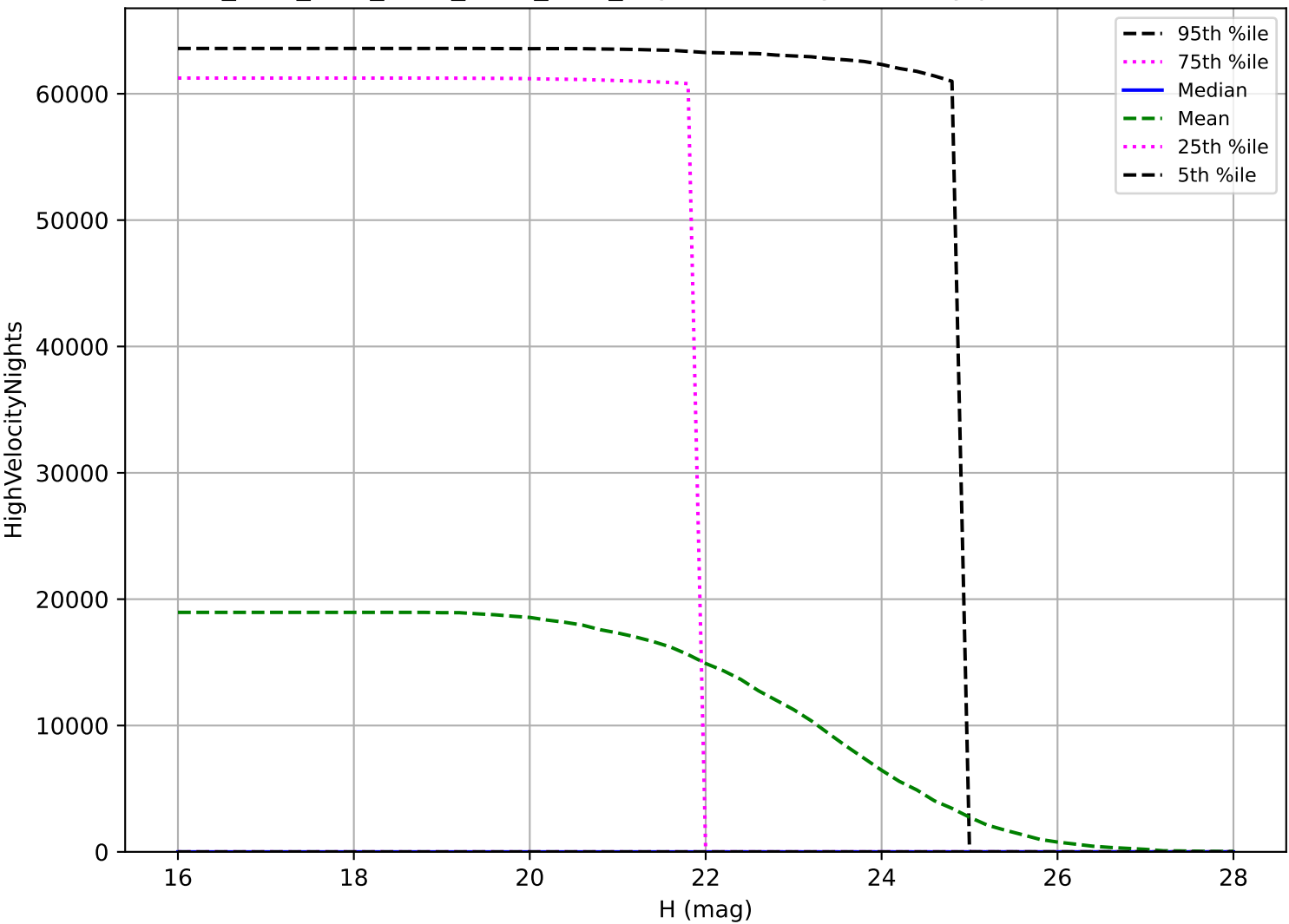
ddf_acor_sf25_lsf30_lsr20_v3.4_10yrs: NEO High velocity pair detection loss
