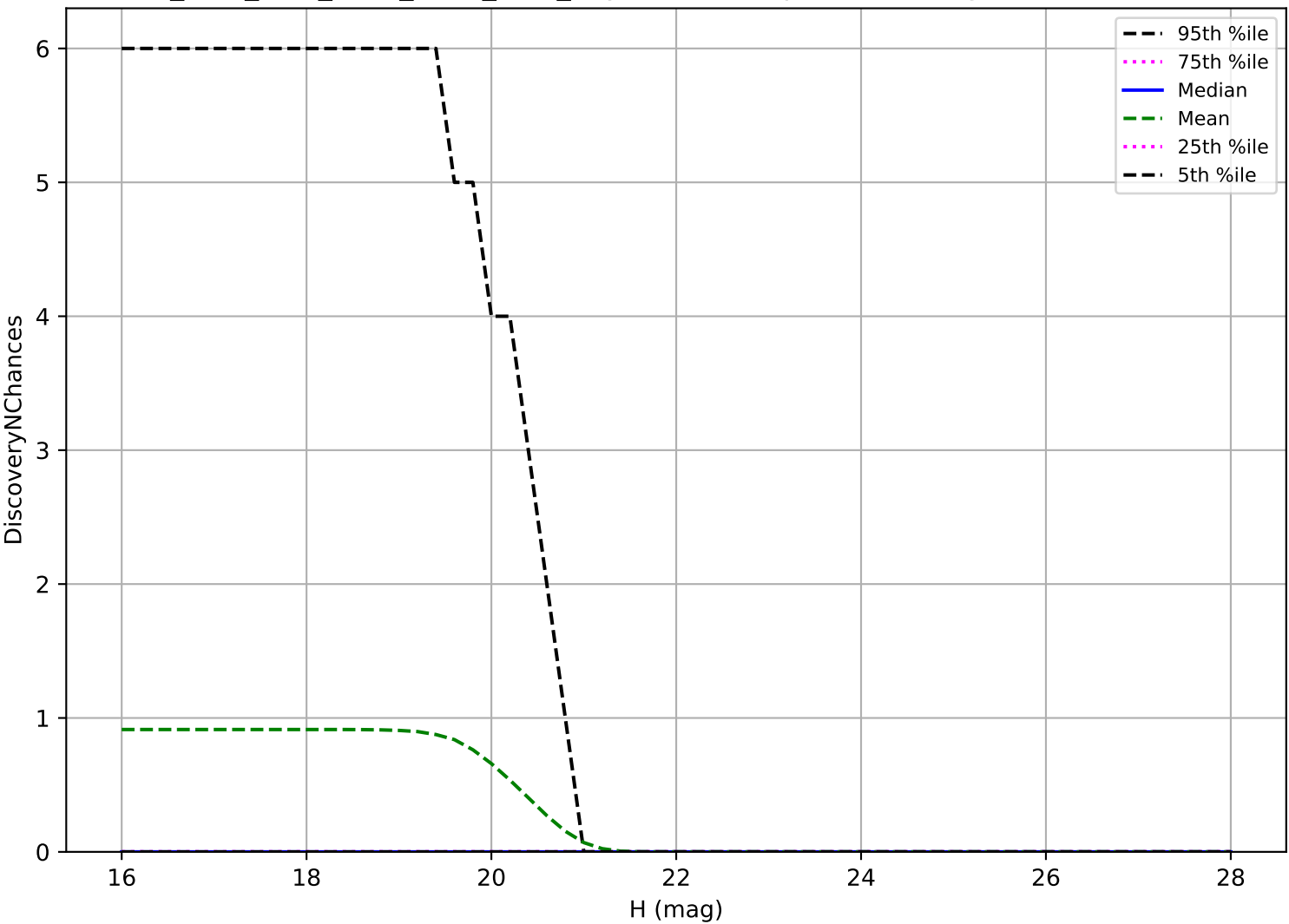
ddf_acor_sf25_lsf30_lsr20_v3.4_10yrs: Vatira 3 pairs in 15 nights detection loss
