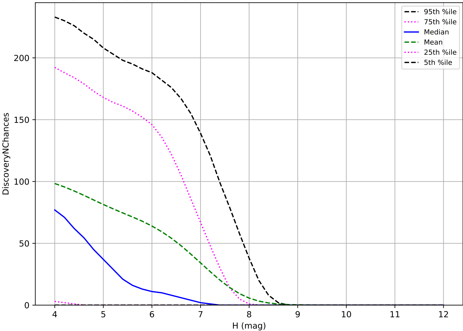
ddf_acor_sf25_lsf30_lsr20_v3.4_10yrs: TNO 3 pairs in 15 nights detection loss
