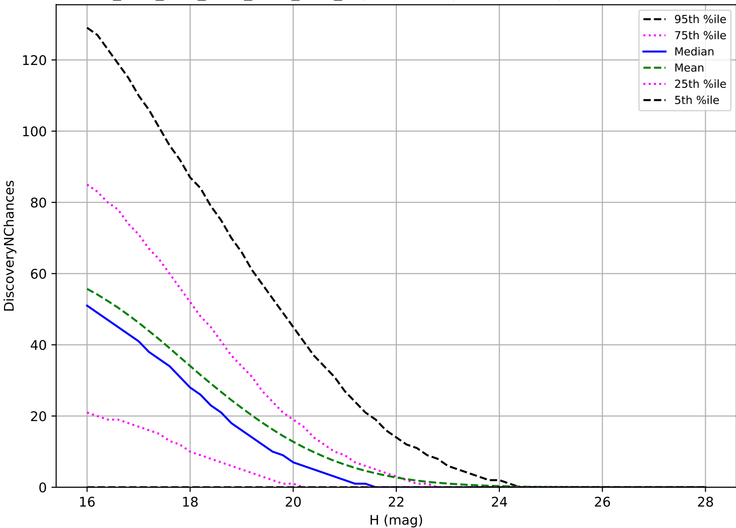
ddf_acor_sf25_lsf30_lsr20_v3.4_10yrs: NEO 3 pairs in 15 nights detection loss
