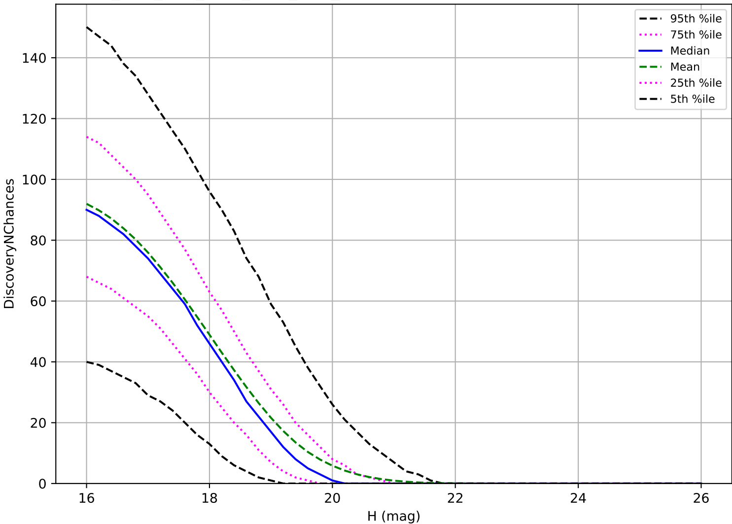
ddf_acor_sf25_lsf30_lsr20_v3.4_10yrs: MBA 3 pairs in 15 nights detection loss
