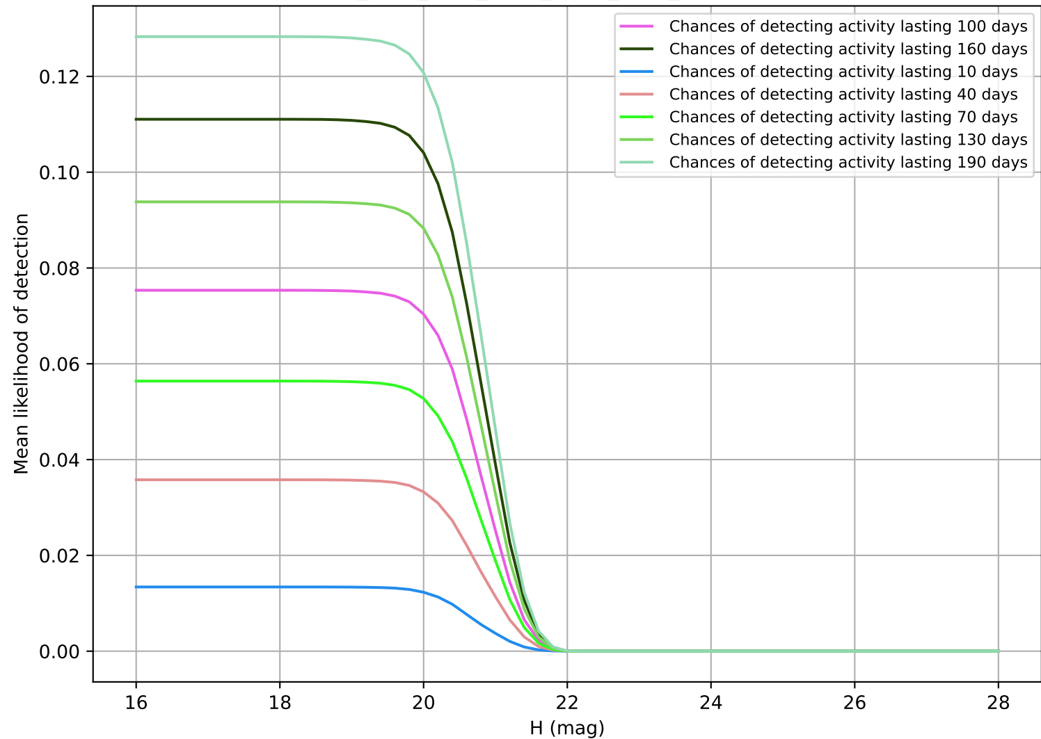
ddf_acor_sf25_lsf30_lsr20_v3.4_10yrs Vatira
