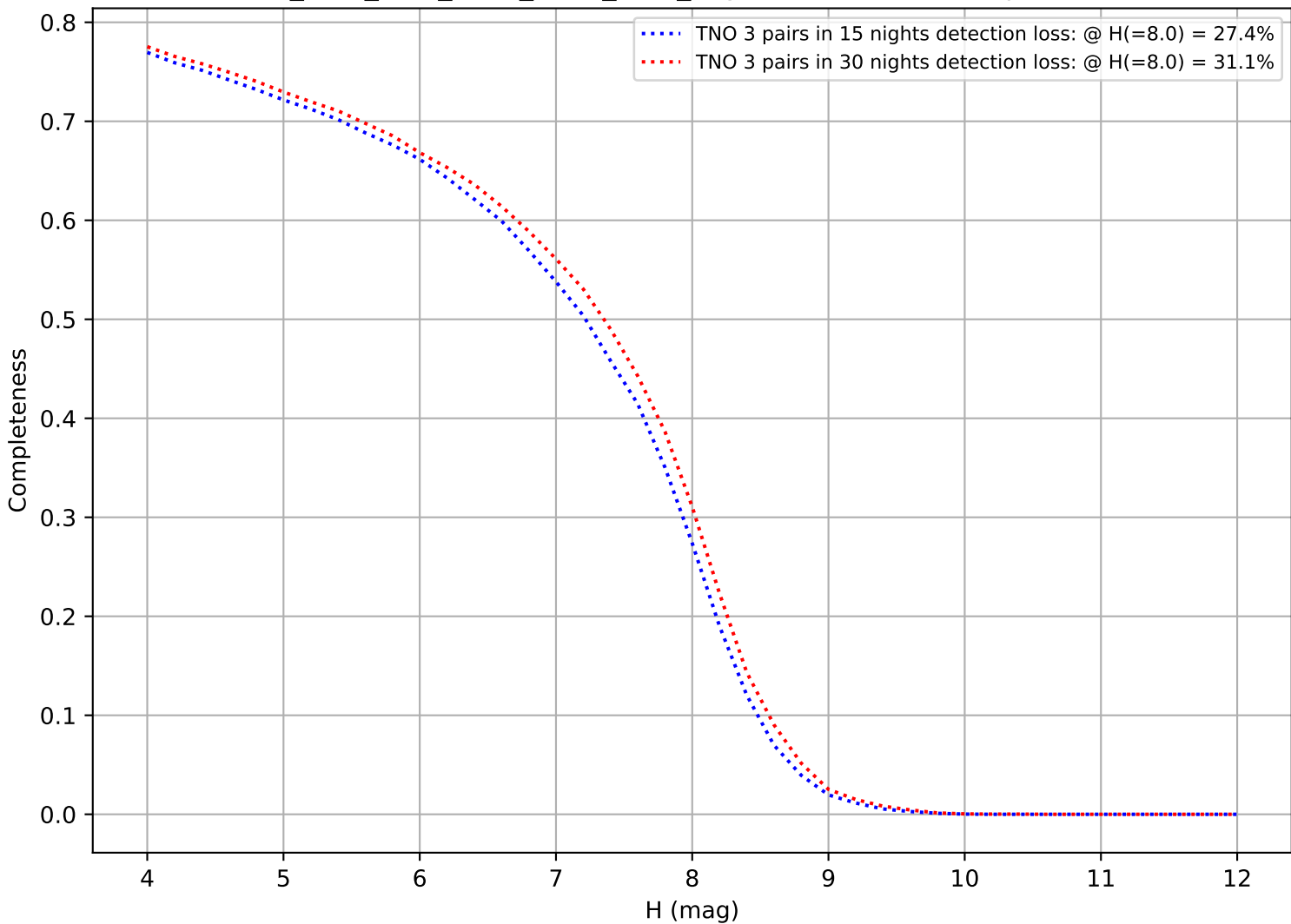
ddf_acor_sf25_lsf30_lsr20_v3.4_10yrs: DifferentialCompleteness
