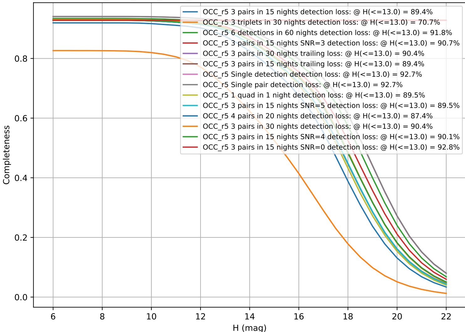
ddf_acor_sf25_lsf30_lsr20_v3.4_10yrs: CumulativeCompleteness
