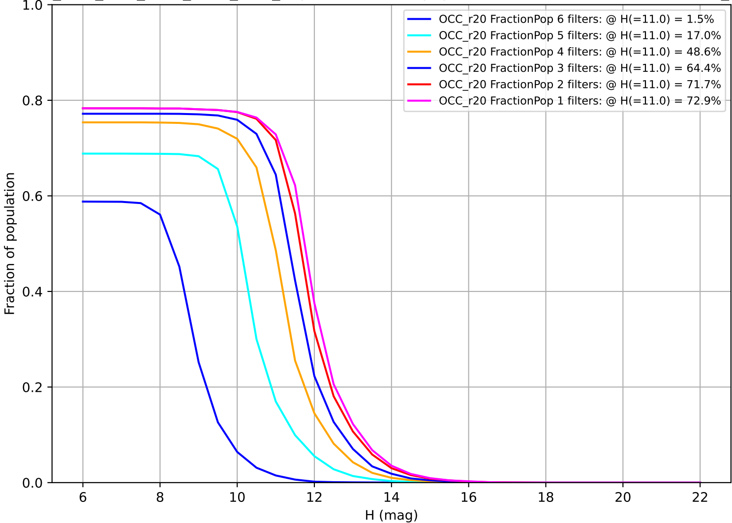
ddf_acor_sf25_lsf30_lsr20_v3.4_10yrs: Fraction of population with colors in X filters OCC_r20
