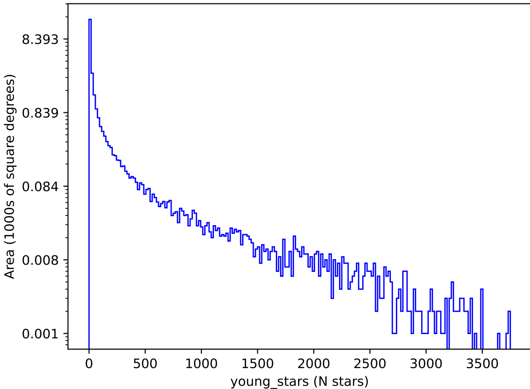
ddf_acor_sf25_lsf30_lsr20_v3.4_10yrs : young_stars
