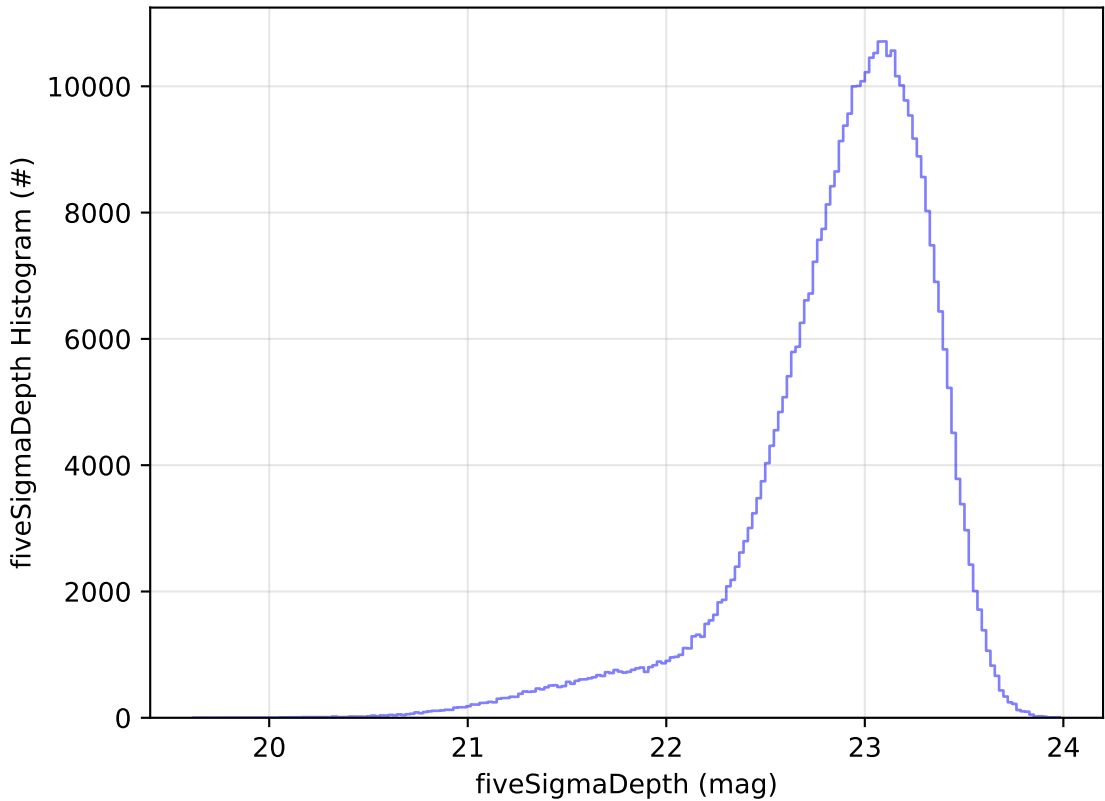
ddf_acor_sf25_lsf30_lsr20_v3.4_10yrs z: fiveSigmaDepth Histogram
