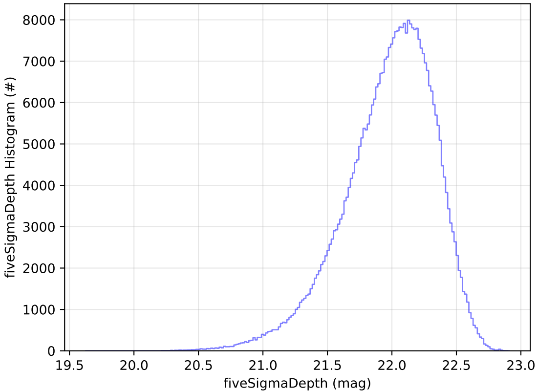
ddf_acor_sf25_lsf30_lsr20_v3.4_10yrs y: fiveSigmaDepth Histogram
